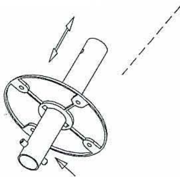
FIXING BASE TO BOTTOM
